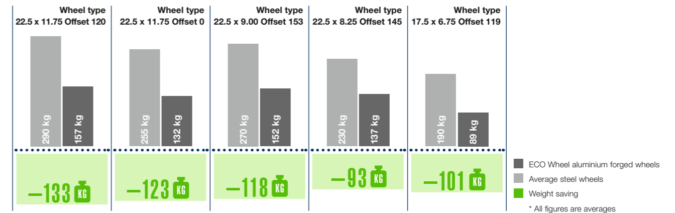
Weight saving due to use of ECO Wheel (using the example of a 3-axle module)
